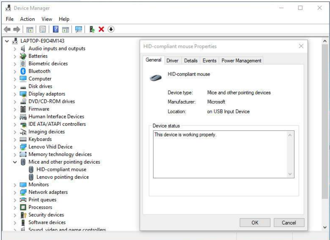
Figure 8.1: Device Manager
