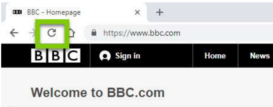
Figure 11.13: Refresh button
