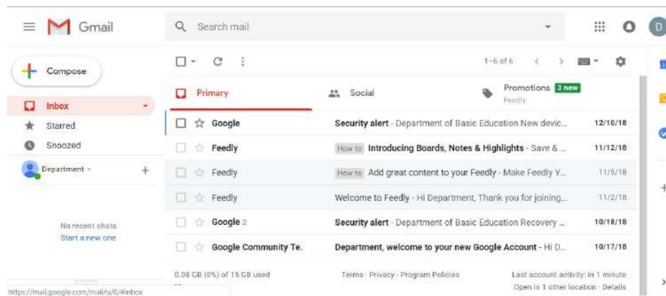
Figure 12.11: Inbox
